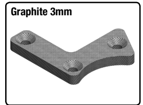
C-00180-235 Suspension arm stiffener - B - Lower Front - Left - 1 pc
