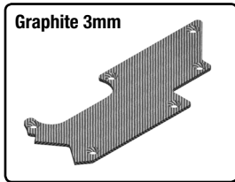
C-00180-236 Suspension arm stiffener - Rear - Right - 1 pc
