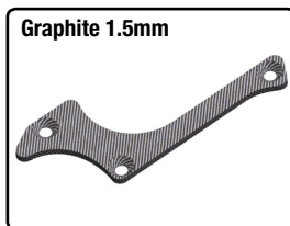
C-00180-273 Suspension arm stiffener - A - Lower Front - Left - 1 pc
