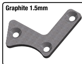
C-00180-274 Suspension arm stiffener - B - Lower Front - Right - 1 pc
